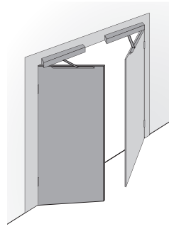
(2-leaf door, master/slave operation) Two electrically coupled drives with standard arm pulling
