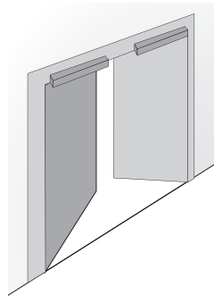
(2-leaf door, master/slave operation) Two electrically coupled drives with standard arm pushing
