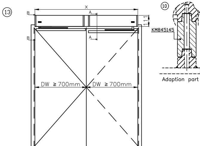
UniSwing Solid Double push/pull (KONE USS-D-P-T)
