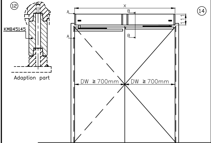
UniSwing Solid Double push/pull (KONE USS-D-P-T)
