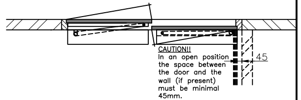
UniSwing Solid Double push/pull (KONE USS-D-P-T)
